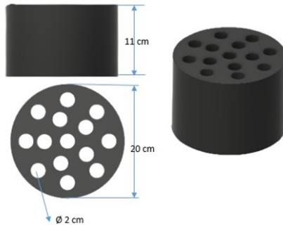
Gambar 2. Prototype briket 14 Lubang
