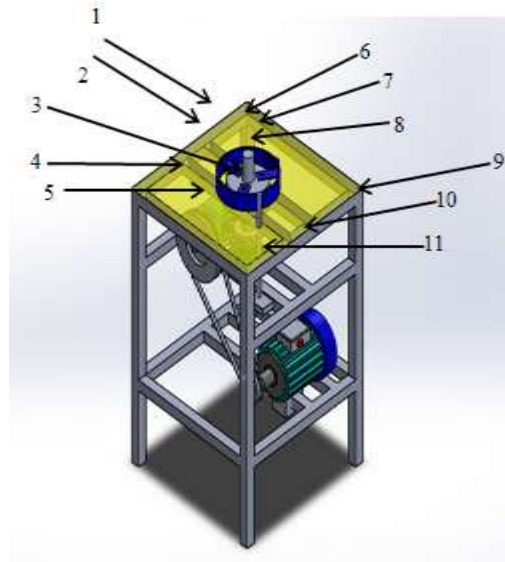
Gambar 3. Mesin Bending Rotary Baja Beton
