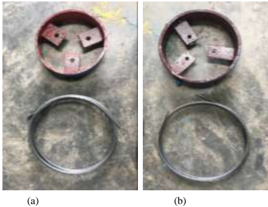
(a) Hasil Bending Mal 8 Inci (b) Hasil Bending Mal 10 Inci
